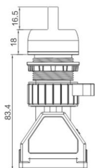
8097-2金属(不锈钢)隔爆防爆控制旋钮 8097-2 type metal (stainless steel) explosion-proof control rotary button
