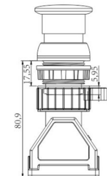
8097防爆防腐控制急停按钮 -不锈钢圈 8097 type explosion-proof emergency stop button - stainless steel ring
