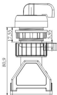
8097防爆防腐控制旋钮开关 -不锈钢圈 8097 type explosion-proof control rotary button - stainless steel ring
