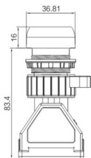
8097-2金属(不锈钢)隔爆防爆控制按钮 8097-2 type metal (stainless steel) explosion-proof control push button
