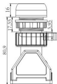
8097防爆防腐控制按钮 -不锈钢圈 8097 type explosion-proof control rotary button - cable type
